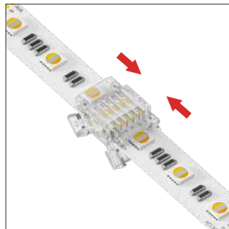
2. Insert Strip Light
