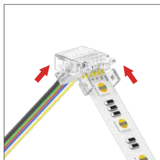
2. Insert Strip Light & Wire
