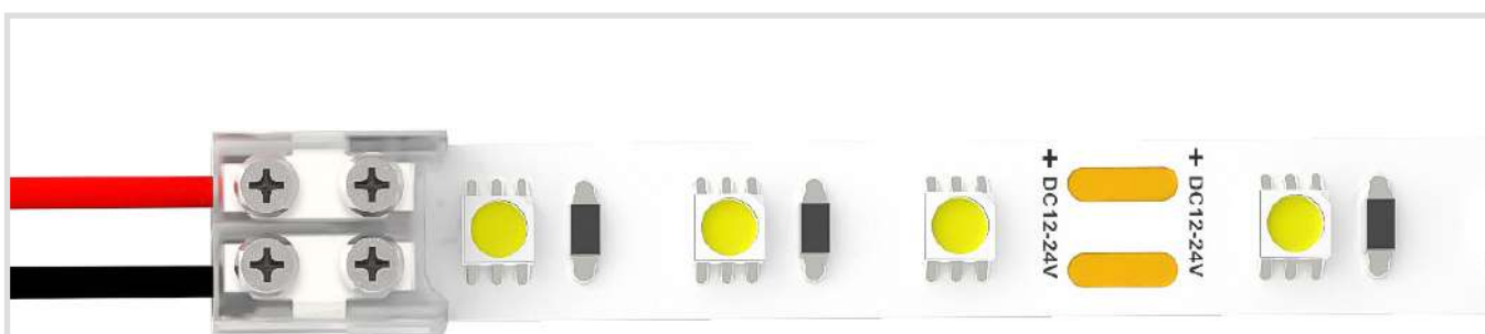
Strip to Wire
